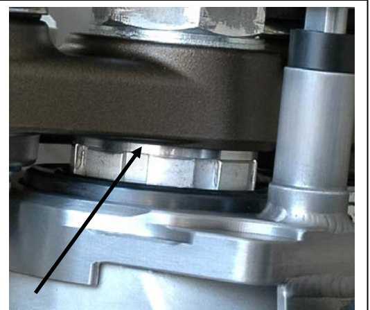
This shows the "spacer-washer" installed on top of the jam nut and under the triple clamp.
