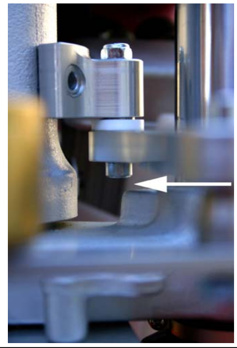
Clearance for the bolt head over the steering stop on the lower triple clamp.
