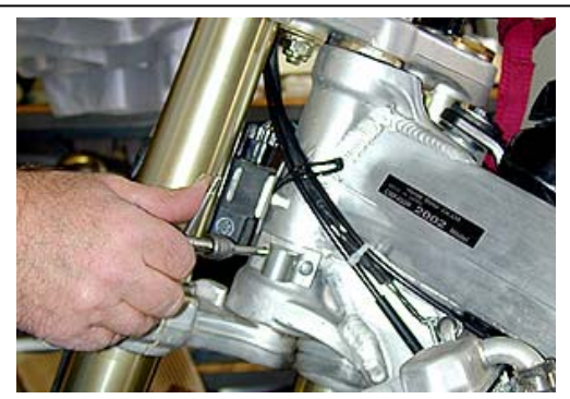
Clearance for the bolt head over the steering stop on the lower triple clamp.
