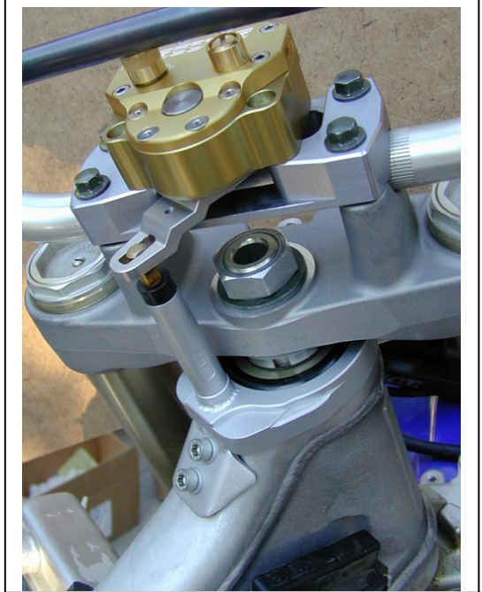
Finished kit showing the stock triple clamp and Renthal bars with a higher crossbar.
