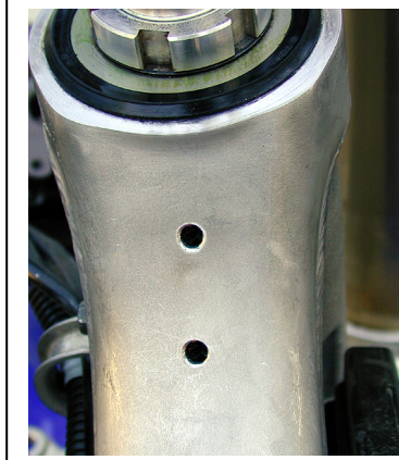
Be sure the frame bracket is all the way down flush with the head tube, all the way around the entire surface.
