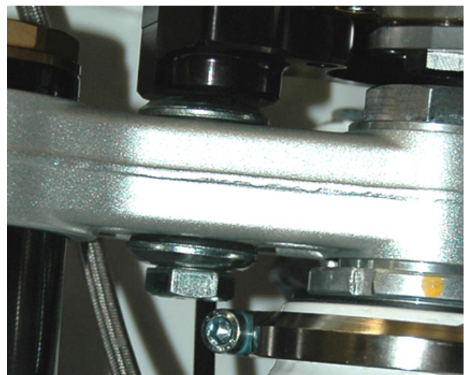
Note the bolt head to frame bracket clearance
