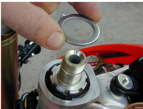
This shows where the spacer goes: under the triple clamp on top of the Jam nut to space it upwards for more clearance. Call if you have questions.
