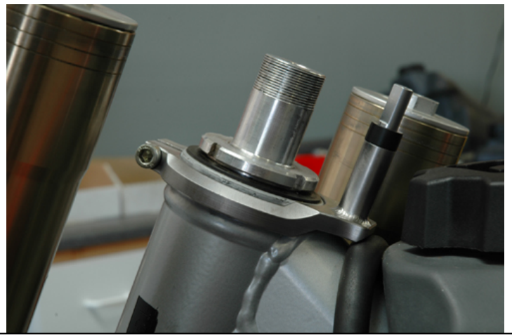
Here is the frame bracket installed, with it low enough to clear the bolt heads on the bottom side of the triple clamp.
