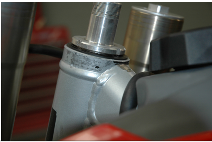
Shown here is some filing at the back of the head tube until the frame bracket is allowed to sit down far enough to clear nuts.
