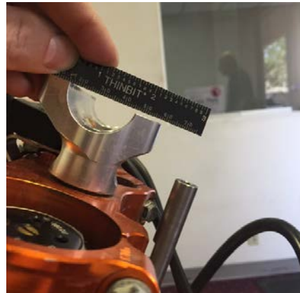
Be sure when using the stock lower cradle that you tighten the high side bolts first. In the reversed position the high side would be toward the rear of the bike.
