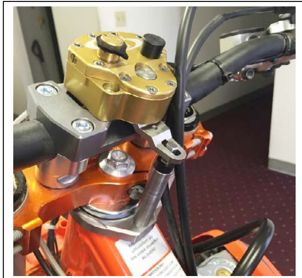
Shown here is the lower Barclamp cradle with the bars in the Forward position. You must tighten the front bolts first, so the Barclamp butts down tightly.
