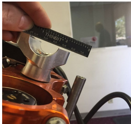
Be sure when using the stock lower cradle that you tighten the high side bolts first. In the reversed position the high side would be toward the rear of the bike.
